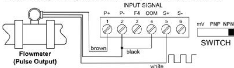
Figure 7: Flowmeter Powered by Internal Power Supply
