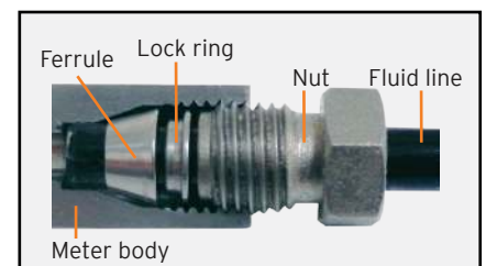
Figure 2. Compression Fitting
